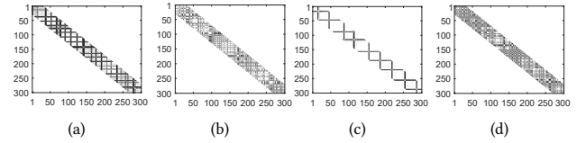
Figure 8: Examples of \mathcal{M}_{\text{dist}} and \mathcal{M}_{\text{orient}} of the k -STGG (with k = 30 ) that is constructed from a sequence of n = 300 gazes: (a) and (b) show the \mathcal{M}_{\text{dist}} and \mathcal{M}_{\text{orient}} when the subject is 'browsing the Internet'; (c) and (d) are the matrices when the subject is 'reading articles'.
