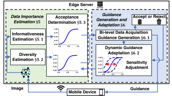
Figure 4: BiGuide System architecture.
