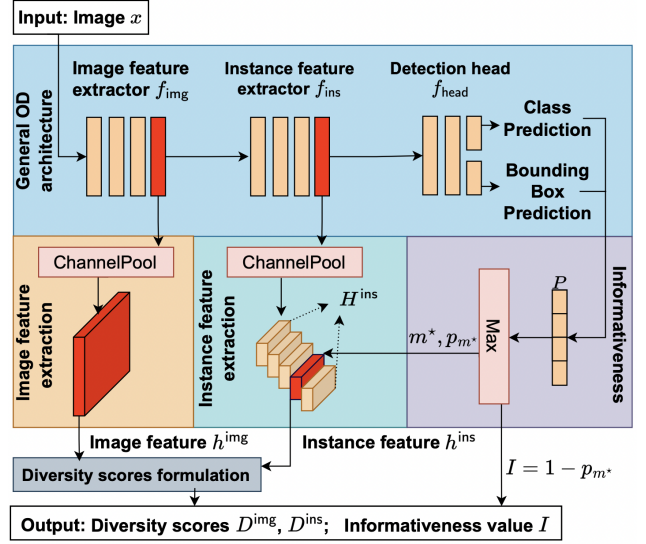
Figure 5: Informativeness and diversity estimations. We obtain the informativeness I based on the prediction confidence and calculate the diversity scores D^{\text{img}} , D^{\text{ins}} based on the image and instance features extracted by the OD model.
